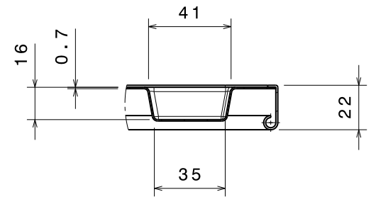
DETALLE "Z"
